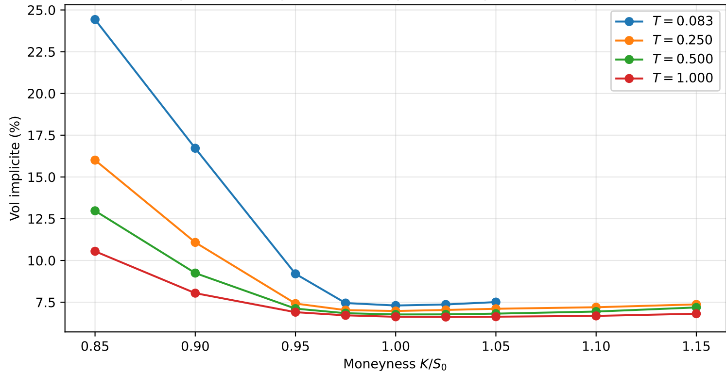
Smile quadratic rough Heston -- asymetrie negative et explosion ATM
