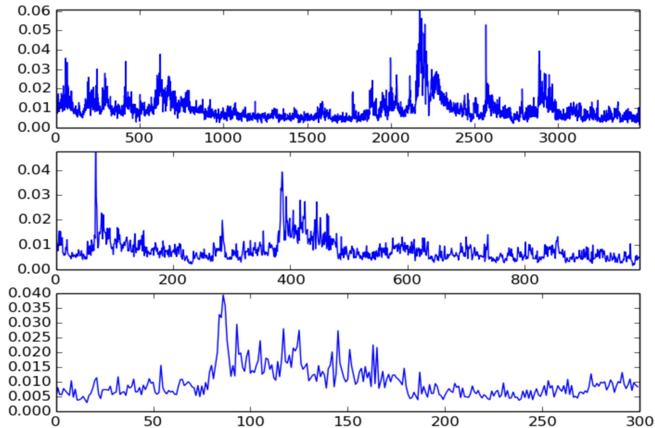
FIGURE : Empirical volatility over 10, 3 and 1 years.
